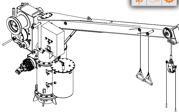
SCH 12-3.5 RESCUE BOAT DAVIT
