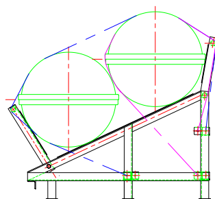
DOUBLE LIFERAFT CONTAINER ROLL-OFF CRADLE
