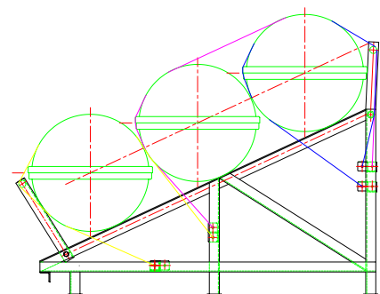
TRIPLE LIFERAFT CONTAINER ROLL-OFF CRADLE
