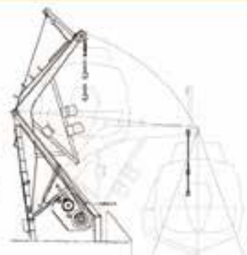
Single Pivot Gravity
